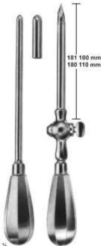
11-198 - 199 Inside dime. Outside dime 11-198 8,5 mm 8,0 mm 11-199 9,0 mm 10,0 mm Empyema trocars
